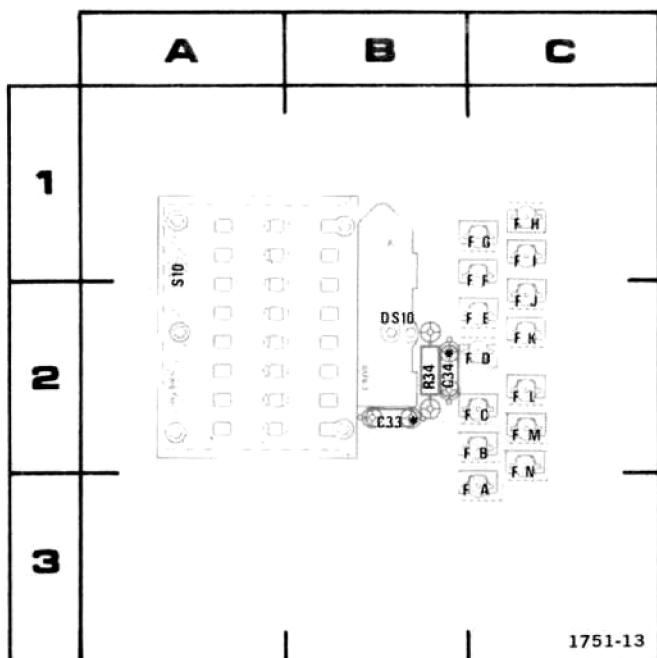
Fig. 8-5. A2—Source Switch Circuit Board.
