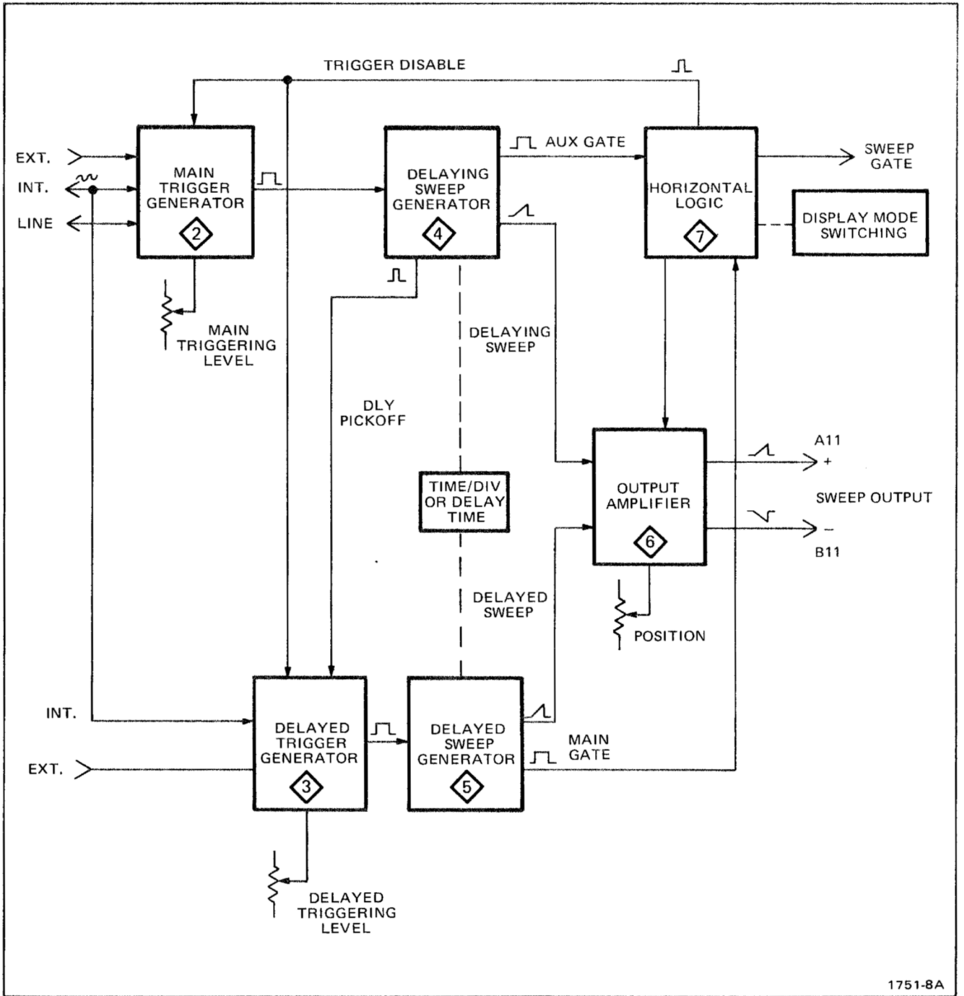
Fig. 8-2. Block Diagram.
