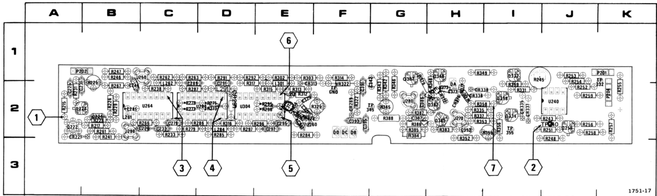
Fig. 8-12. A9-Delayed Trigger Circuit Board (SN B069999 & below).
