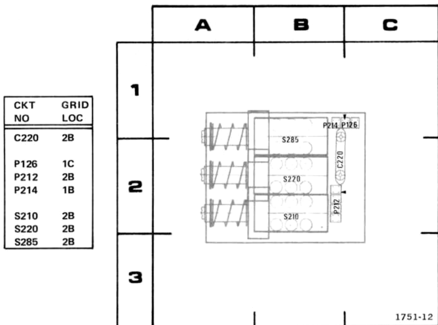
Fig. 8-4. A5—Delayed Triggering Switch Circuit Board.
