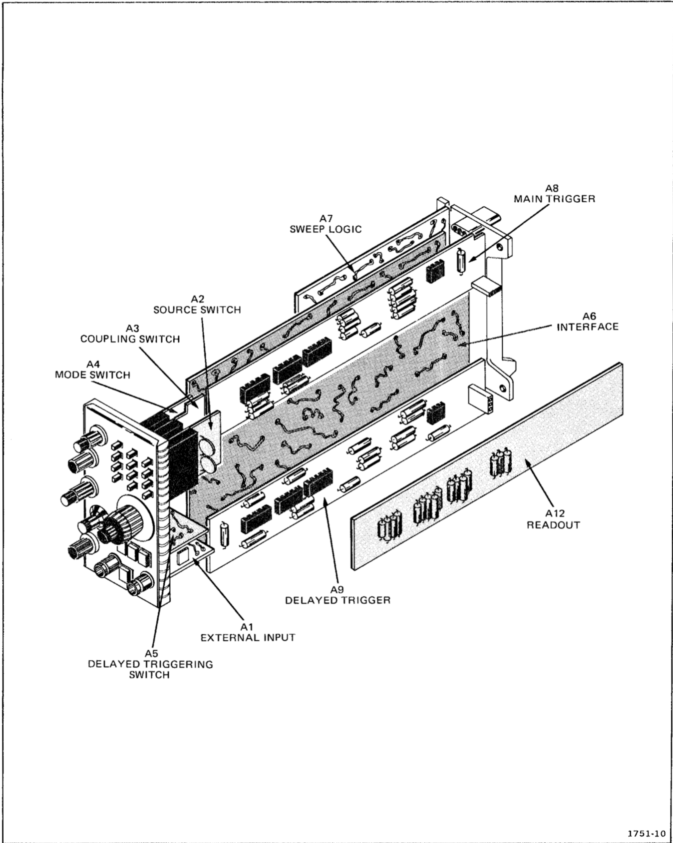
Fig. 8-1. Circuit Board Locations.
