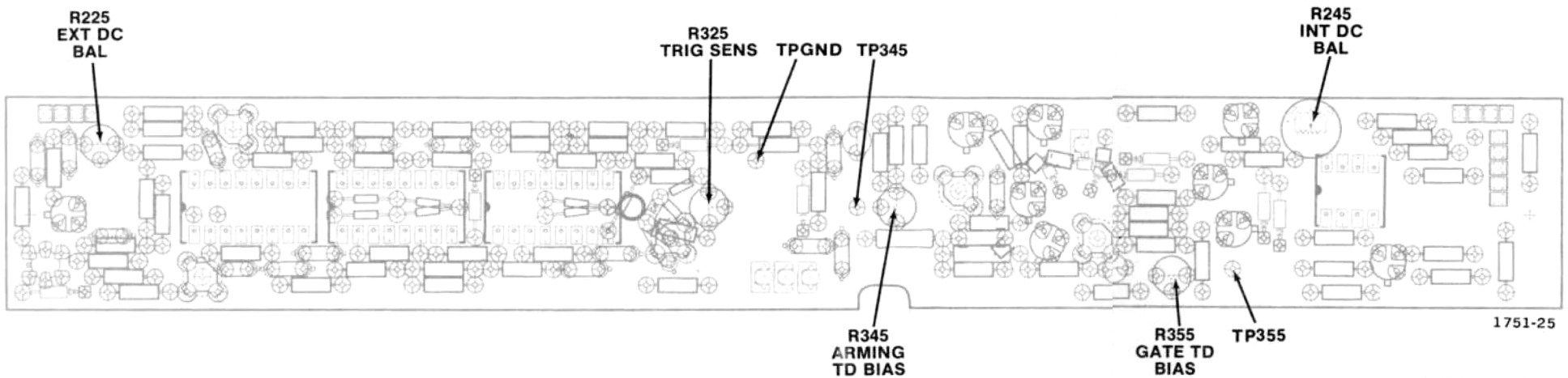
Fig. 8-20. Delayed Trigger Adjustment Location (SN B069999 & below).
