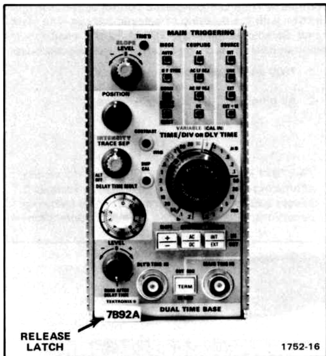
Fig. 1-2. Location of release latch.
