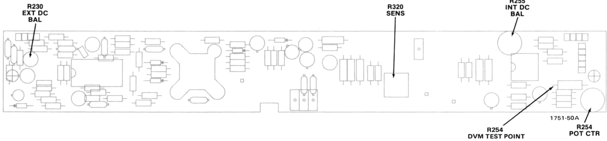
Fig. 8-22. Delayed Trigger Adjustment Location (SN B070000 & up).
