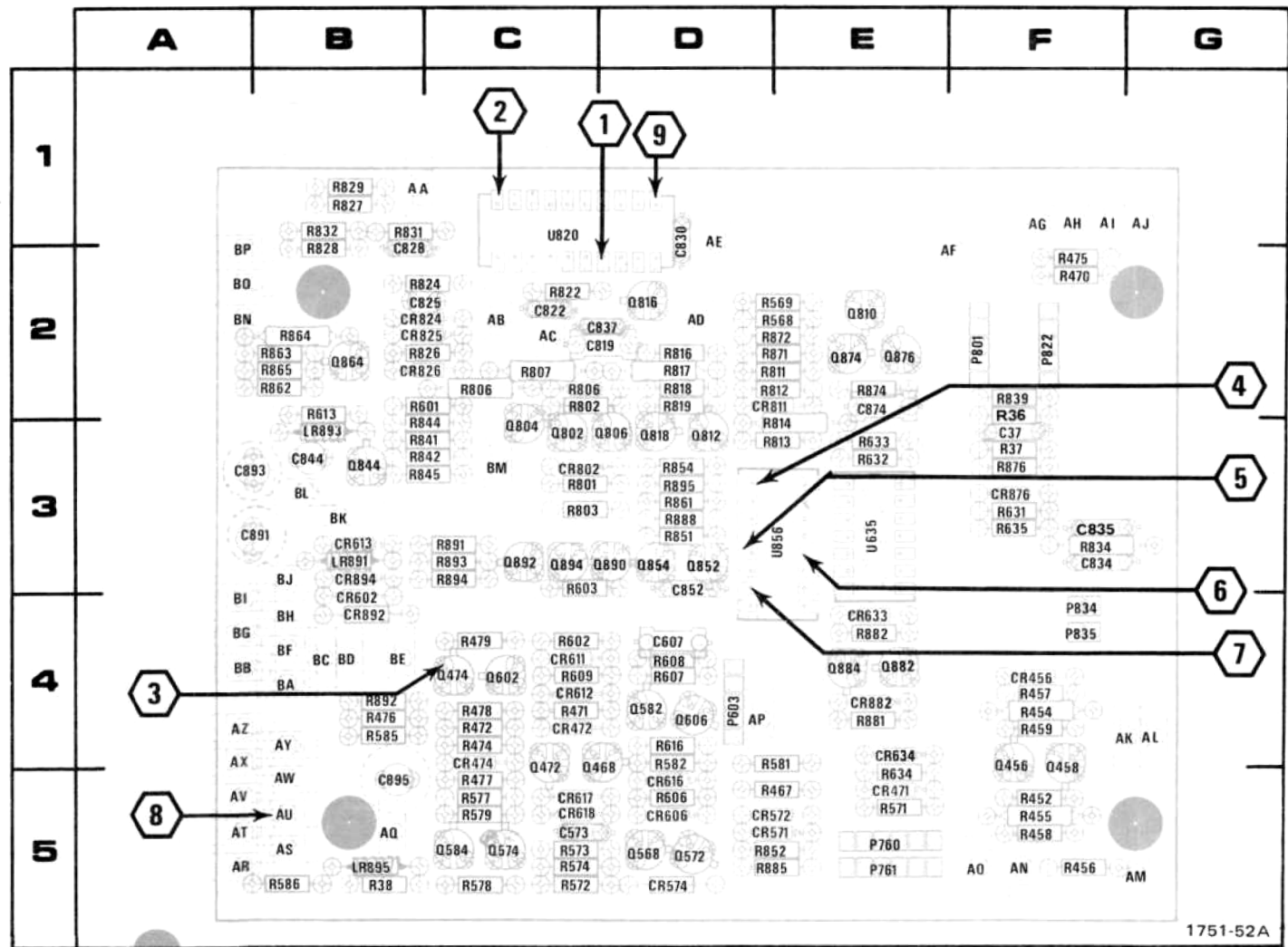
Fig. 8-16. A7-Logic Circuit Board (SN B060000 & up).
